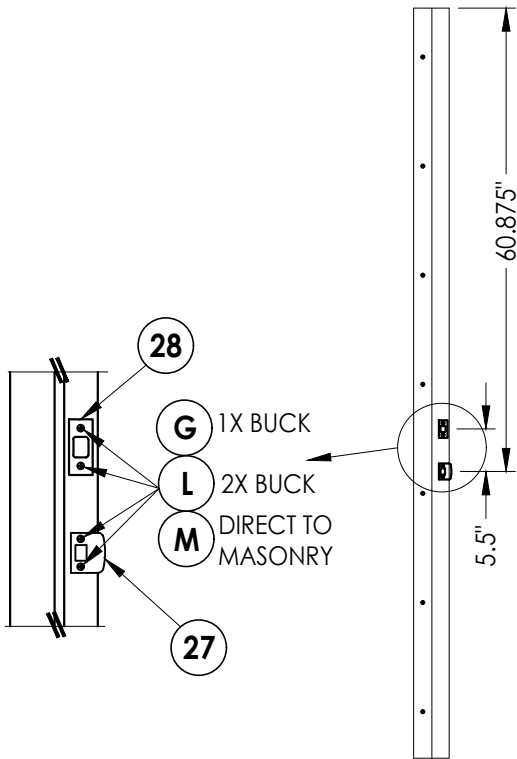
LATCH & DEADBOLT STRIKE PLATE DETAILS
